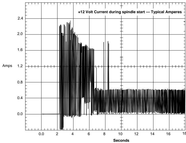
Figure 2. Typical 12V startup and operation current profile
