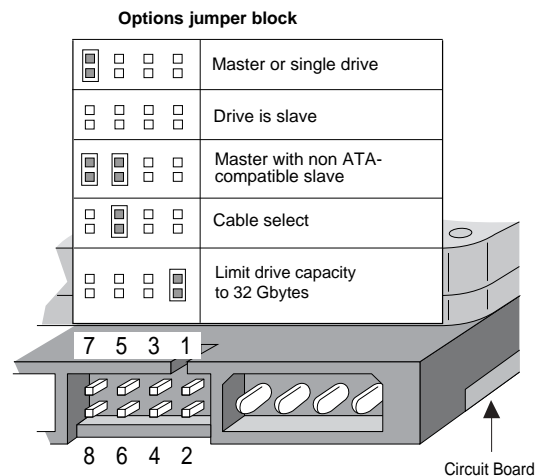
Figure 1. Master/slave jumper settings
